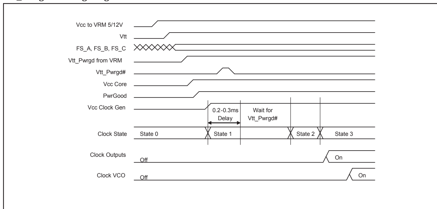
Figure 1. CPU power BEFORE clock power
