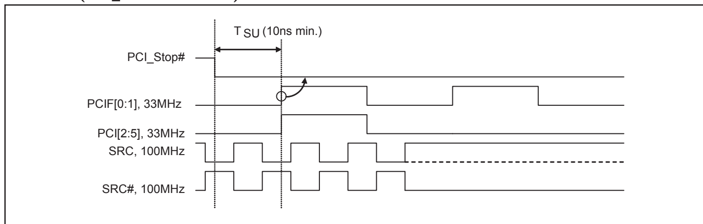
Figure 8. Assertion of PCI_STOP# Waveform
