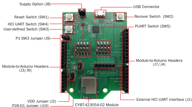
Figure 1: CYBT-423054-EVAL Top View
