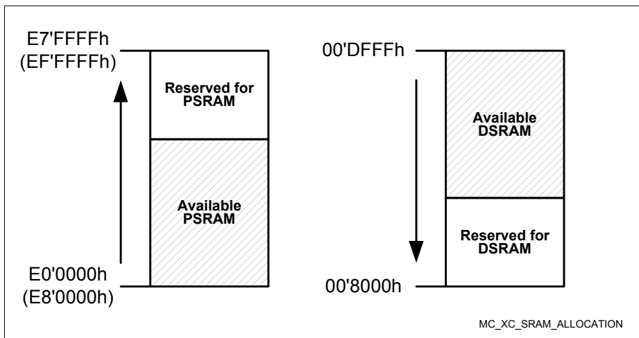
Figure 1 SRAM Allocation
