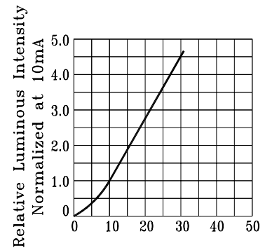
Forward Current (mA) Fig.4 Relative Luminous Intensity vs. Forward Current
