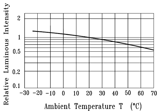
Ambient Temperature T (°C) Fig.5 Luminous Intensity vs. Ambient Temperature
