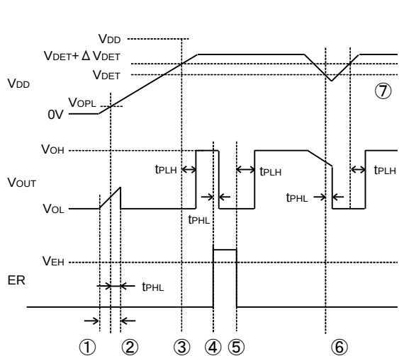
Fig.17 Timing Waveform
