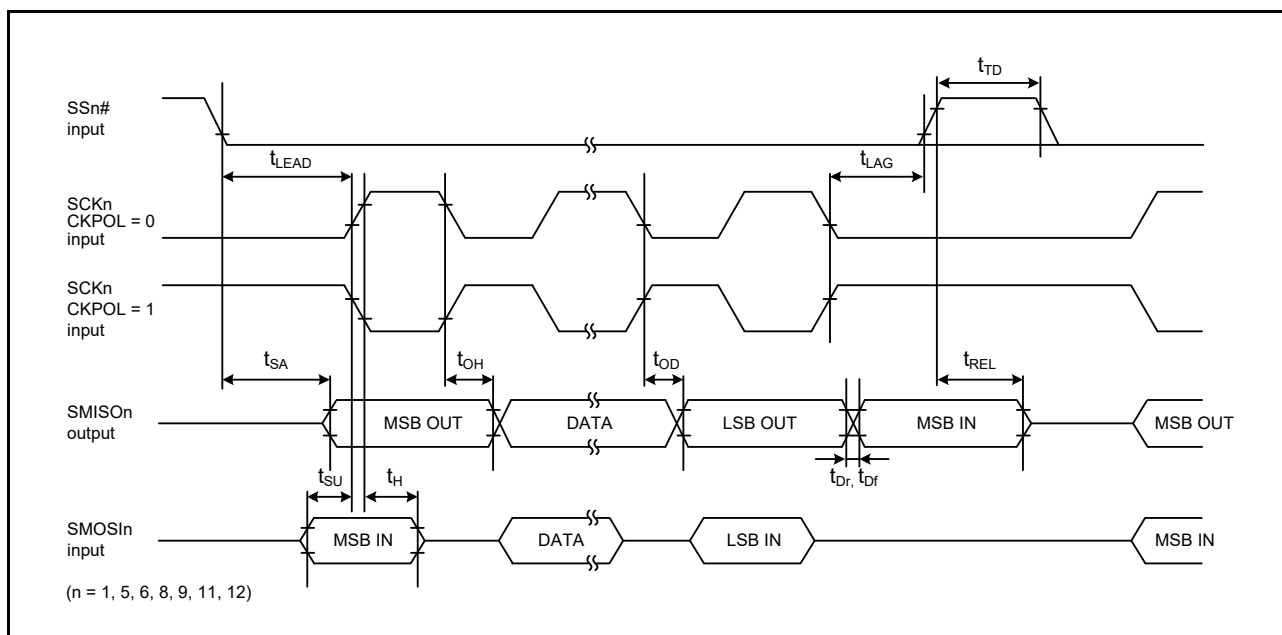
Figure 2.51 Simple SPI Timing (Slave, CKPH = 1)
