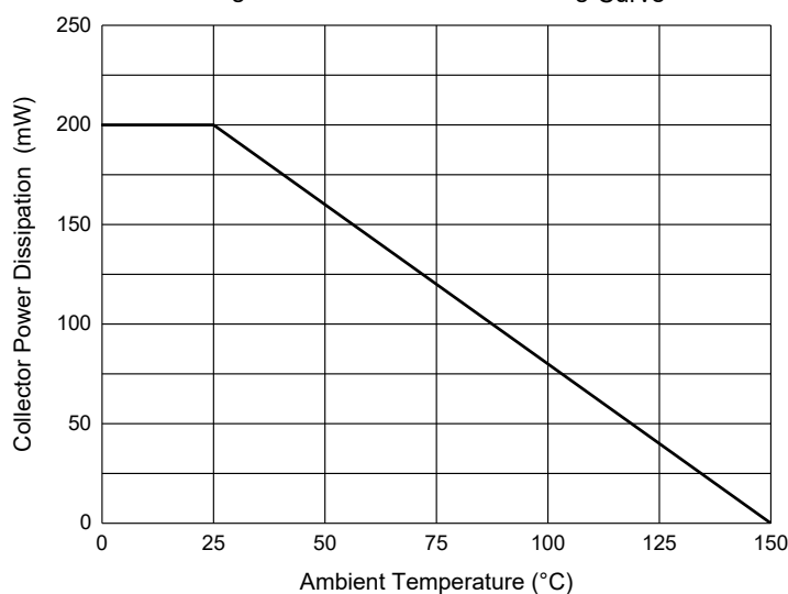
Fig. 12- Collector Power Derating Curve
