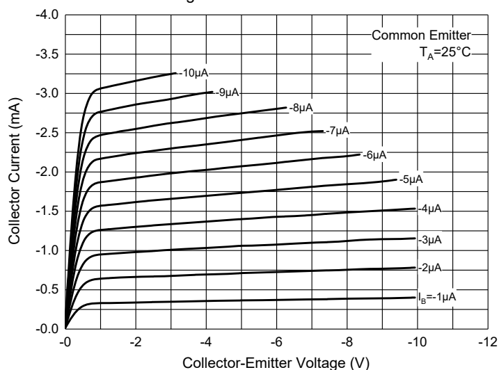
Fig. 7 - Static Characteristics
