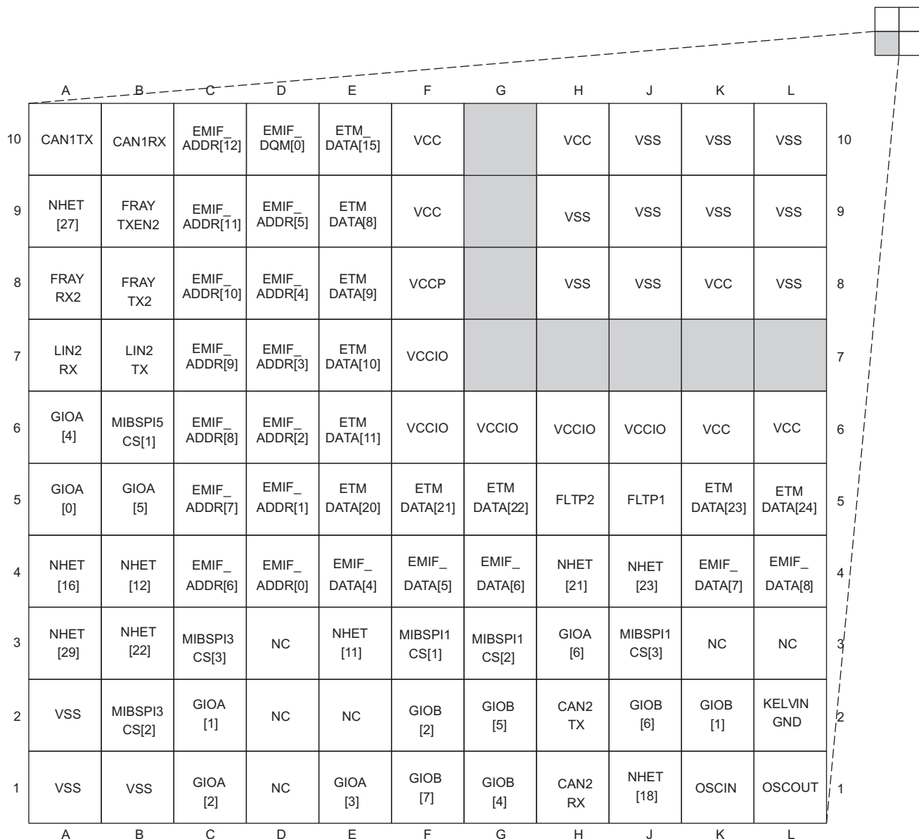
Figure 2-7. ZWT Package Pinout Bottom Left Quadrant (337 ball) [Top View]
