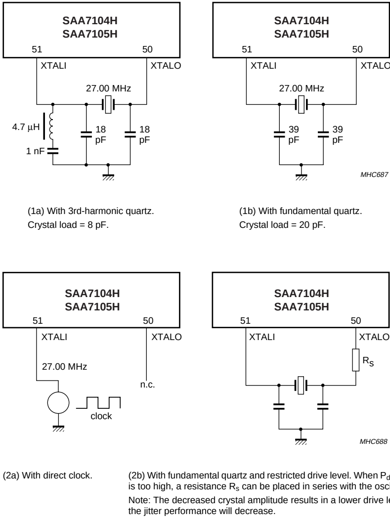
Fig.18 Oscillator application.
