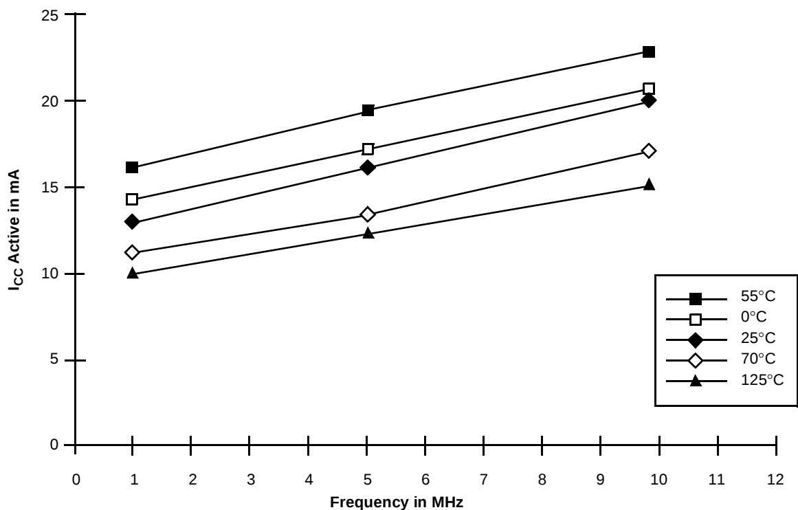
Figure 5. Am28F010—Average I_{CC} Active vs. Frequency
