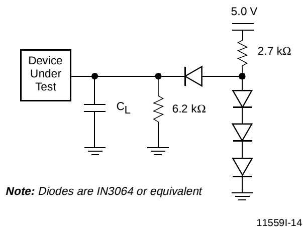
Figure 6. Test Setup
