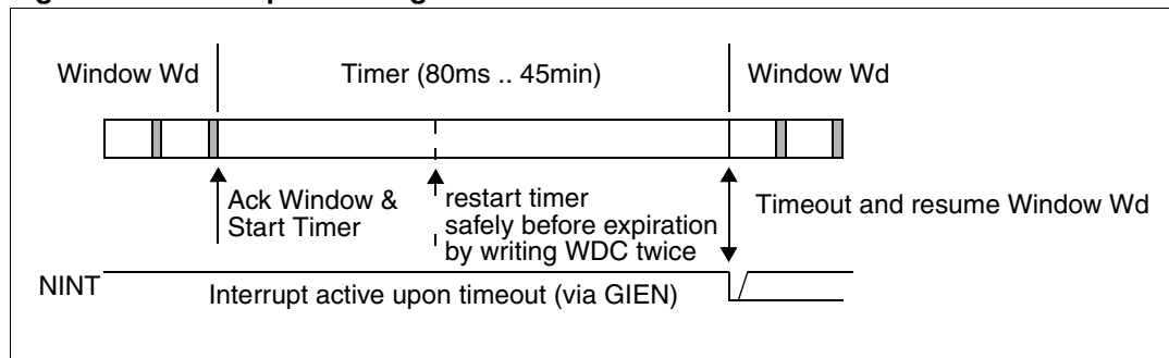
Figure 21. Wakeup watchdog
