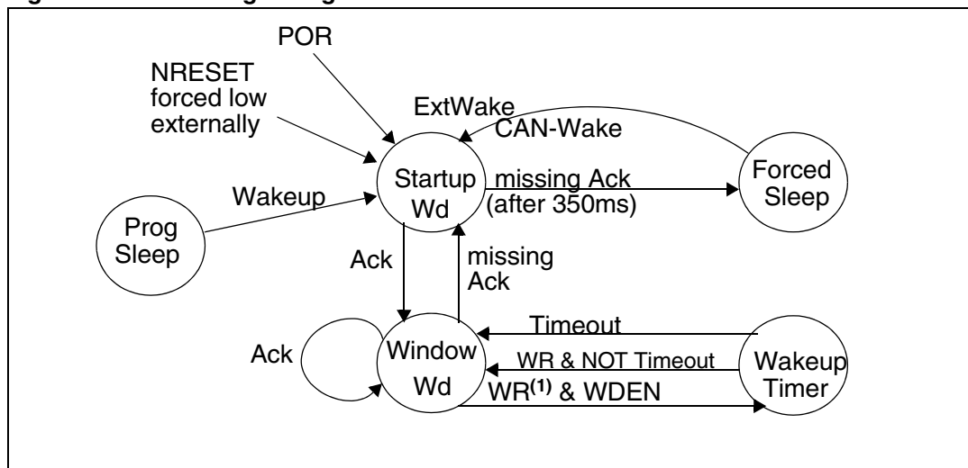
Figure 18. Watchdog configuration
