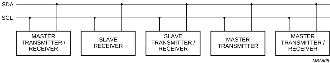
Fig.7 System configuration.
