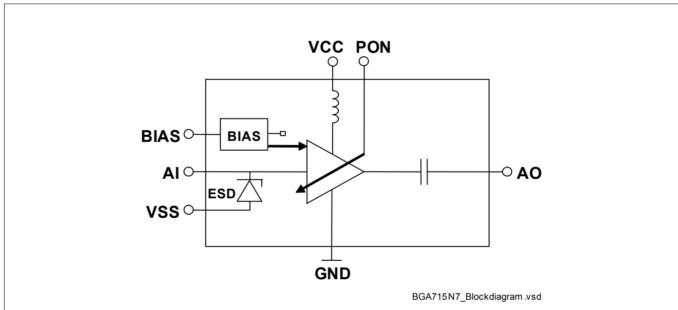
Figure 1 Block Diagram
