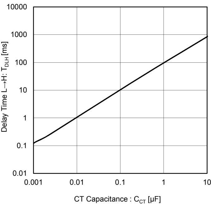
Figure 14. Delay Time L→H vs. CT Capacitance
