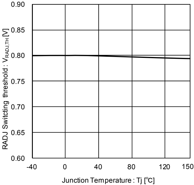
Figure 16. RADJ switching threshold vs. Junction Temperature
