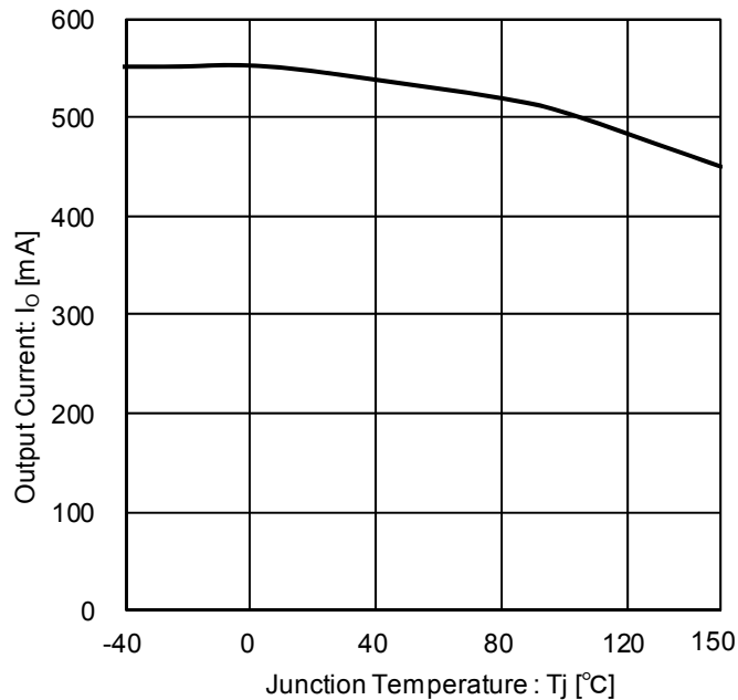
Figure 8. Output Current vs. Junction Temperature
