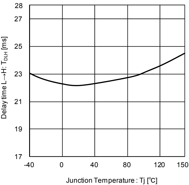
Figure 13. Delay Time L→H vs. Junction Temperature (CCT = 0.22 μF)
