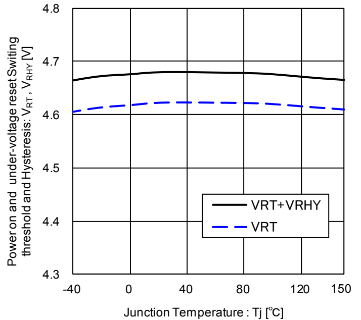
Figure 12. Power on and under-voltage reset Switg threshold and Hysteresis vs. Junction Temperature
