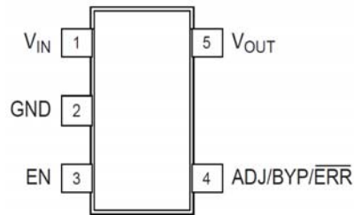
Figure 2. Pin Configuration
