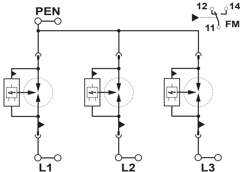
Circuit diagram
