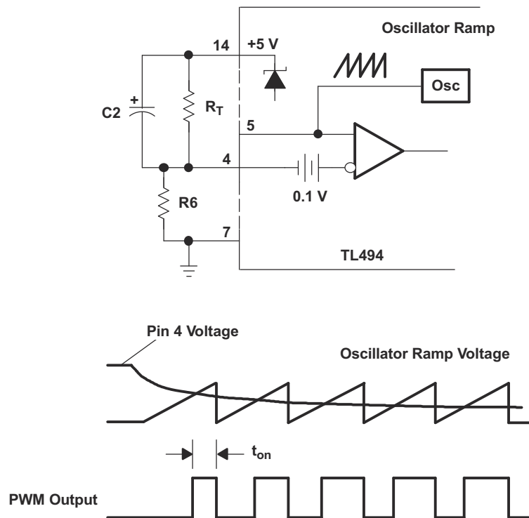
Figure 10-5. Soft-Start Circuit
