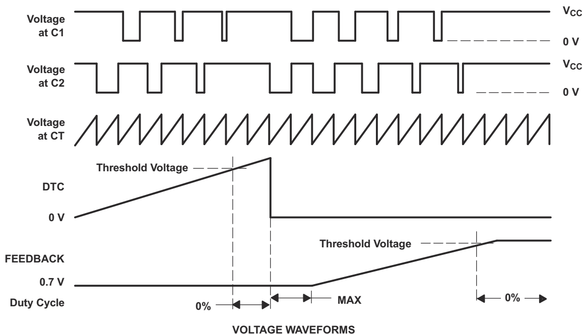
Figure 8-1. Operational Test Circuit and Waveforms
