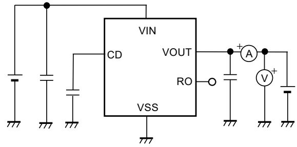
Figure 8 Test Circuit 2
