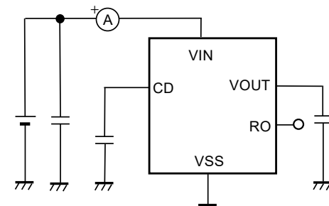
Figure 12 Test Circuit 6
