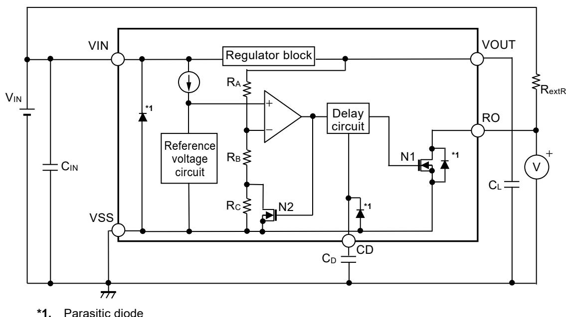
Figure 20 Operation
