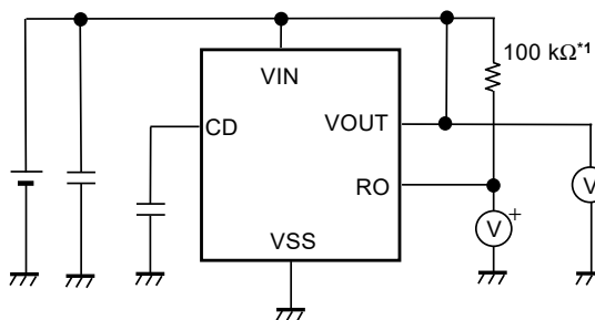
Figure 9 Test Circuit 3
