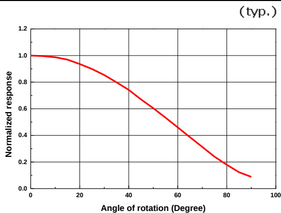
Fig.7 Angular response
