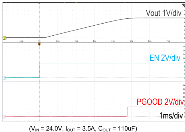
( V_{IN} = 24.0V , I_{OUT} = 3.5A , C_{OUT} = 110\mu F ) Figure 25. On/Off Enable Waveform
