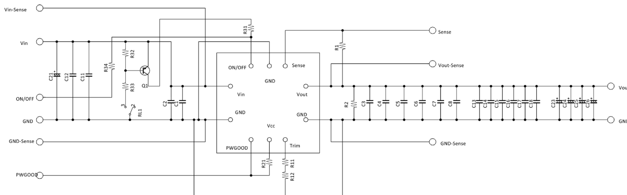
Figure 34. Application Circuit
