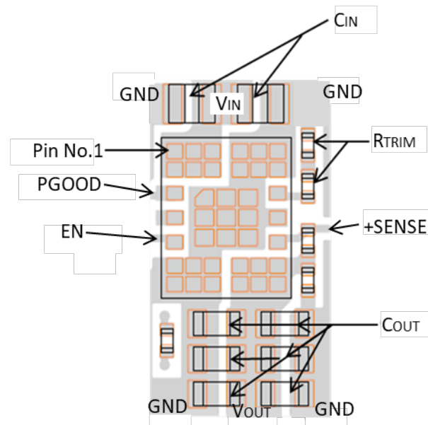
Figure 35. Example of Pattern Layout (Top View)
