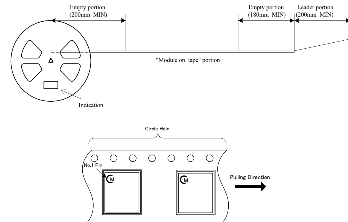
Figure 41. Tape Specifications
