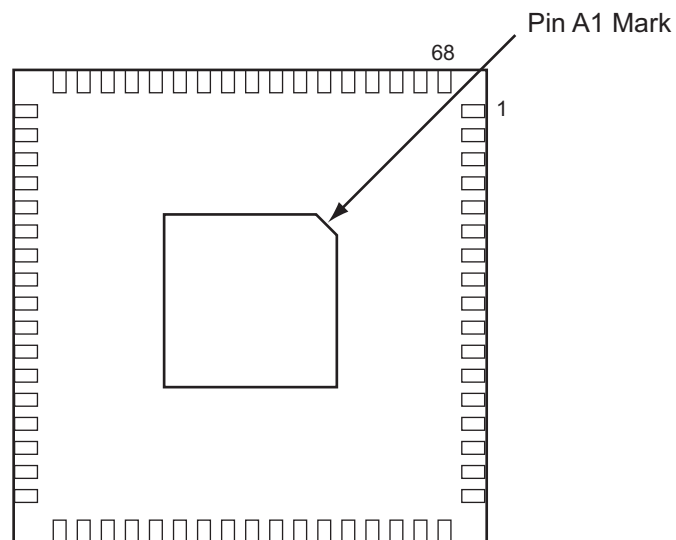
FIGURE 4-7: QN68—BOTTOM-VIEW
