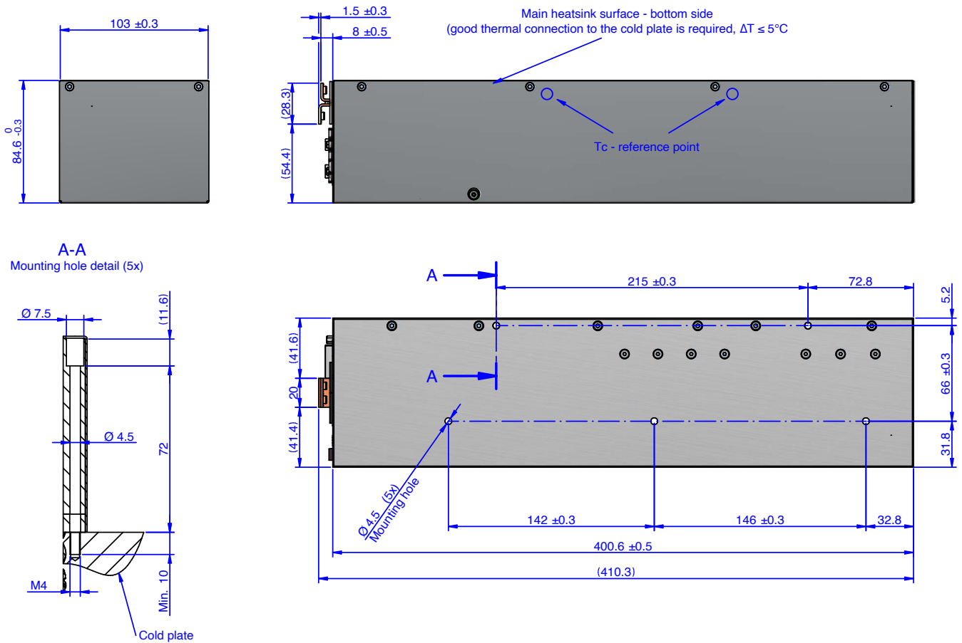
Figure 3. Mechanical Drawing
