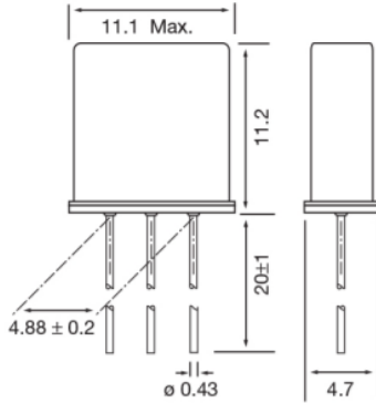
Figure 1) HC-49/U
