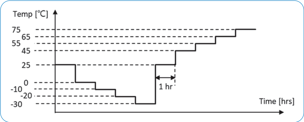
Figure 5: Temperature Characteristics Test
