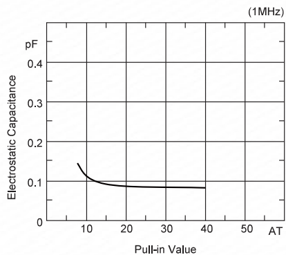
Electrostatic capacitance
