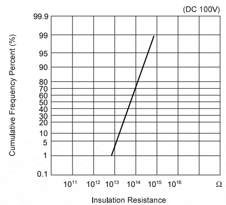
Insulation resistance
