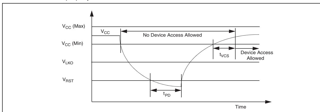
Figure 21 Power down or voltage drop
