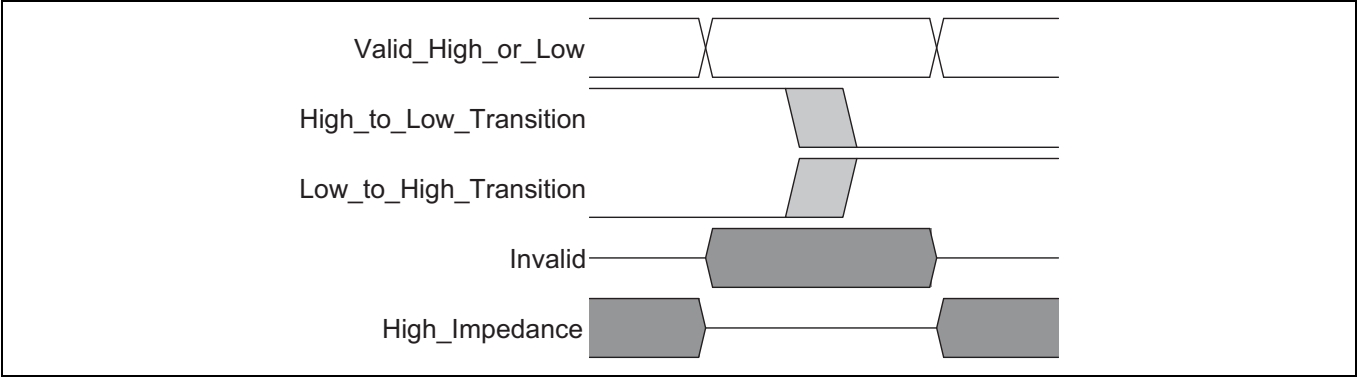
Figure 23 Switching waveforms
