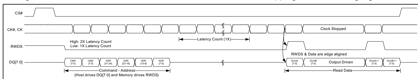
Figure 12 Active clock stop during read transaction (DDR) [44]
