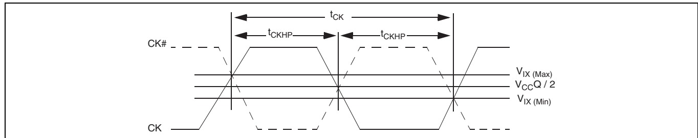
Figure 28 Clock characteristics
