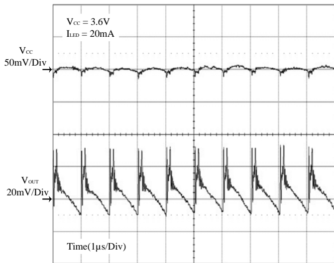
Figure 9 Ripple Voltage
