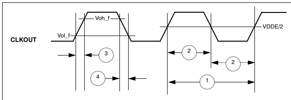
Figure 18. CLKOUT timing
