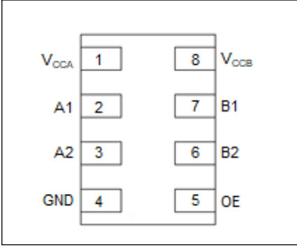
UDFN-8 (TOP VIEW)
