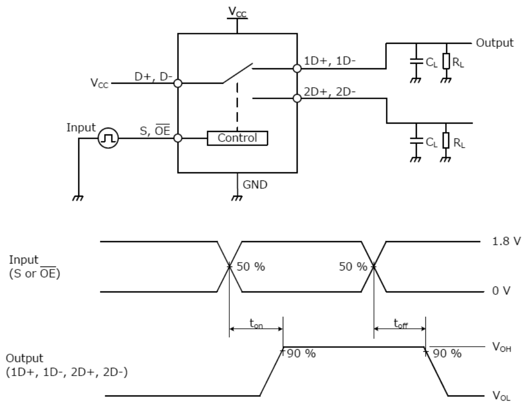
Fig. 11.2 Turn-ON and Turn-OFF Times ( t_{on} , t_{off} )
