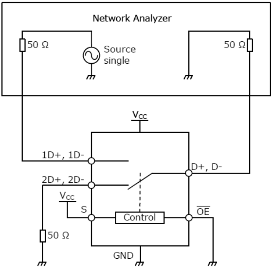
Fig. 11.6 OFF Isolation
