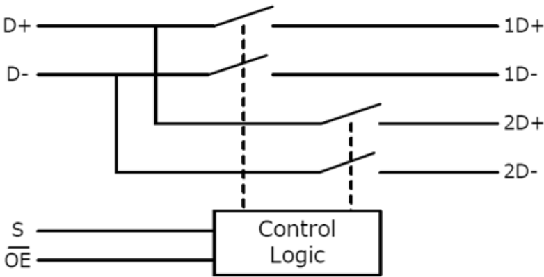
Fig. 6.1 Block Diagram
