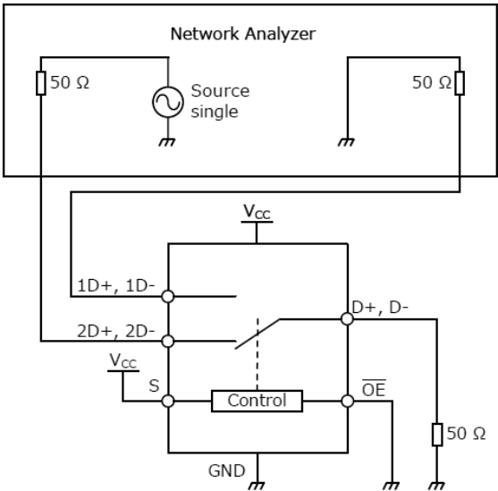
Fig. 11.7 Crosstalk
