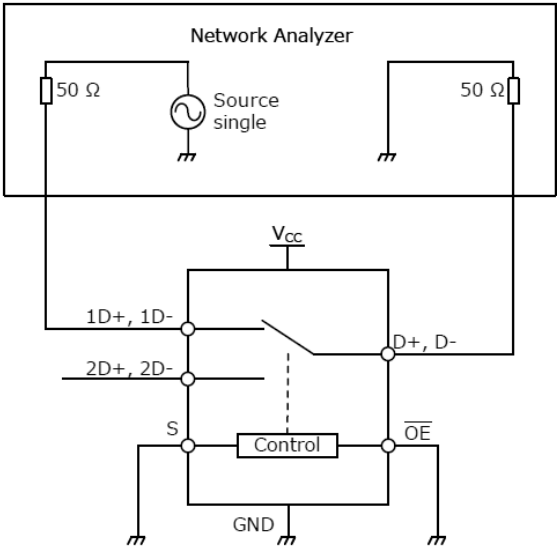
Fig. 11.8 -3dB Bandwidth
