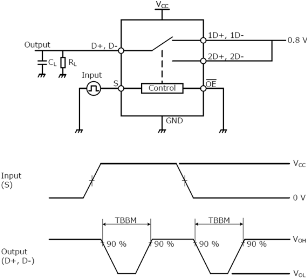
Fig. 11.3 Break Before Make (TBBM)
