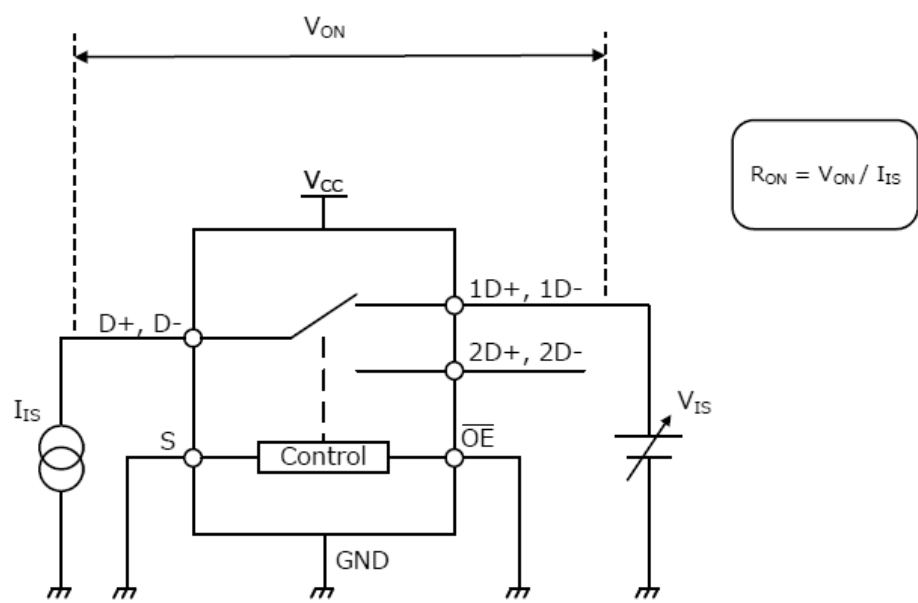
Fig. 11.9 ON-Resistance
