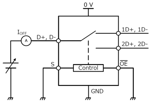
Fig. 11.10 Power-OFF Leakage Current
