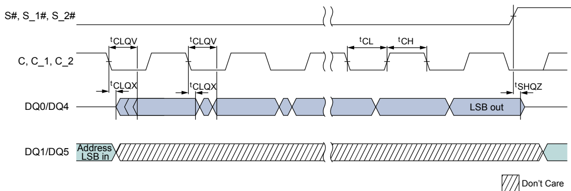
Figure 52: Output Timing
