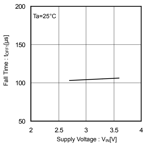
Figure 22. Output Fall Time vs Supply Voltage
