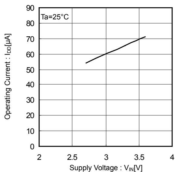
Figure 4. Operating Current vs Supply Voltage (EN Enable)
