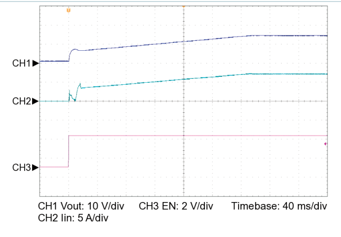
Figure 15 — Startup from EN, V_{IN} = 48\text{ V} , C_{OUT\_EXT} = 10000\text{ }\mu\text{F} , R_{LOAD} = 0.703\text{ }\Omega
