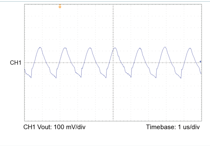
Figure 17 — Output voltage ripple, V_{IN} = 48\text{ V} , V_{OUT} = 15.0\text{ V} , C_{OUT\_EXT} = 1000\text{ }\mu\text{F} , R_{LOAD} = 0.703\text{ }\Omega
