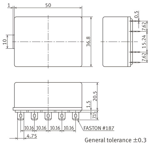
External dimensions
