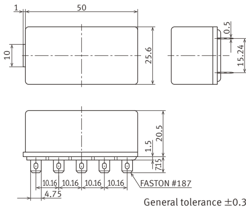
External dimensions
