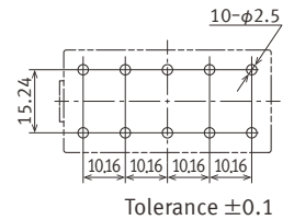
Schematic ( BOTTOM VIEW ) Single side stable ( De-energize )
