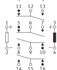
2 coil latching ( Reset )
