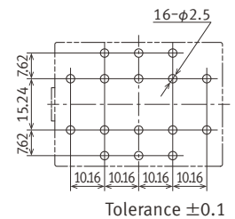
Schematic ( BOTTOM VIEW ) Single side stable ( De-energize )
