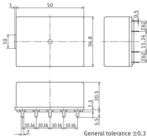
External dimensions
