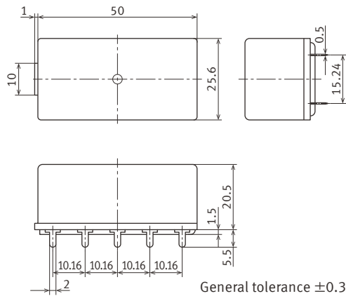
External dimensions
