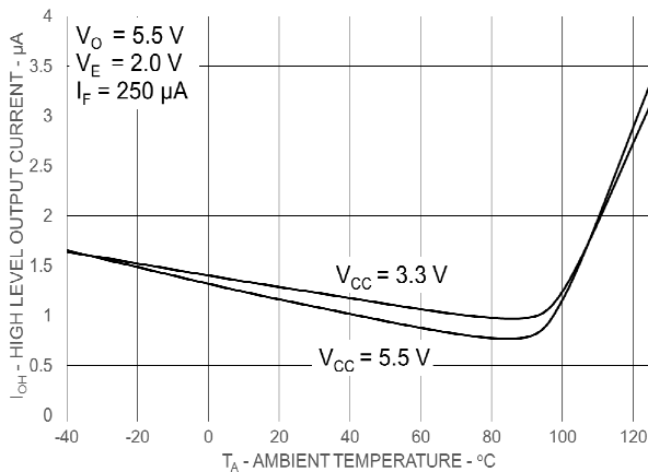
Figure 3: Typical High Level Output Current vs. Ambient Temperature
