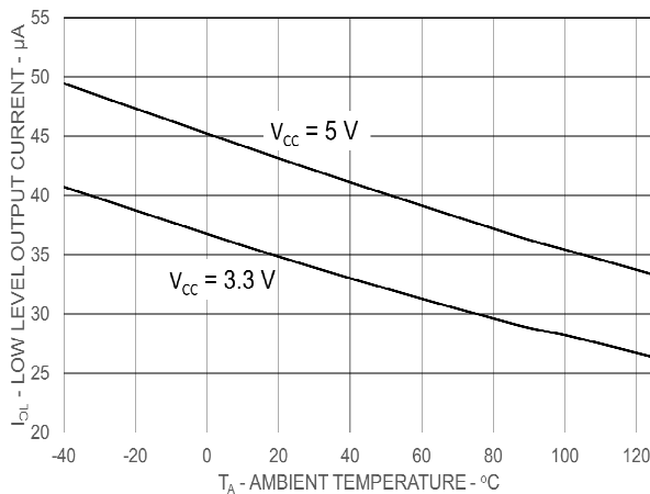
Figure 6: Typical Low Level Output Current vs.
