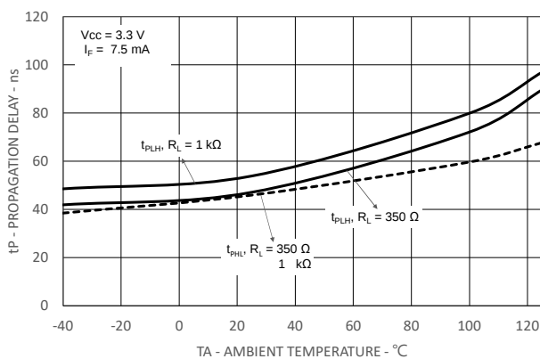
Figure 8: Typical Propagation Delay vs. Ambient Temperature
