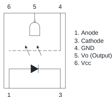
Pin No. and Internal connection diagram
