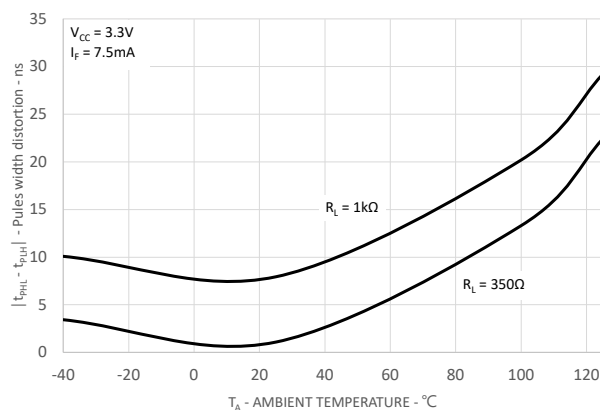
Figure 9: Typical Pulse Width Distortion vs. Ambient Temperature
