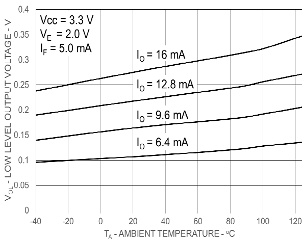
Figure 5: Typical Low Level Output Voltage vs. Ambient Temperature
