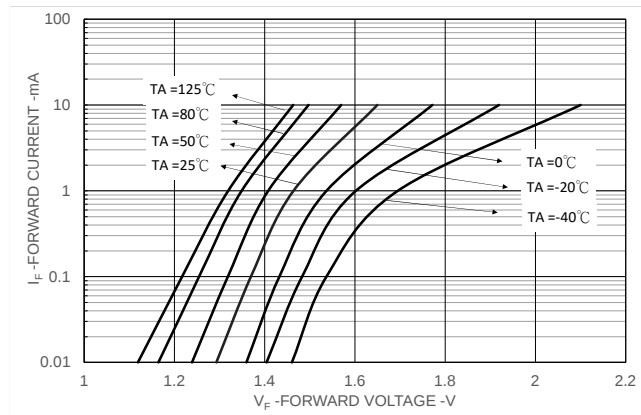
Figure 7: Typical Input Diode Forward Characteristic
