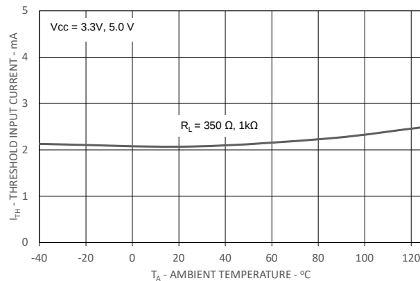
Figure 4: Typical Input Diode Threshold Current vs. Ambient Temperature
