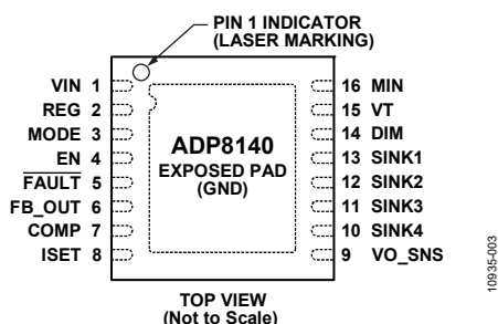
Figure 3. Pin Configuration
