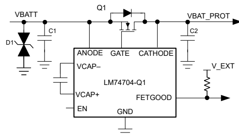
LM74704-Q1 Typical Application Schematic
