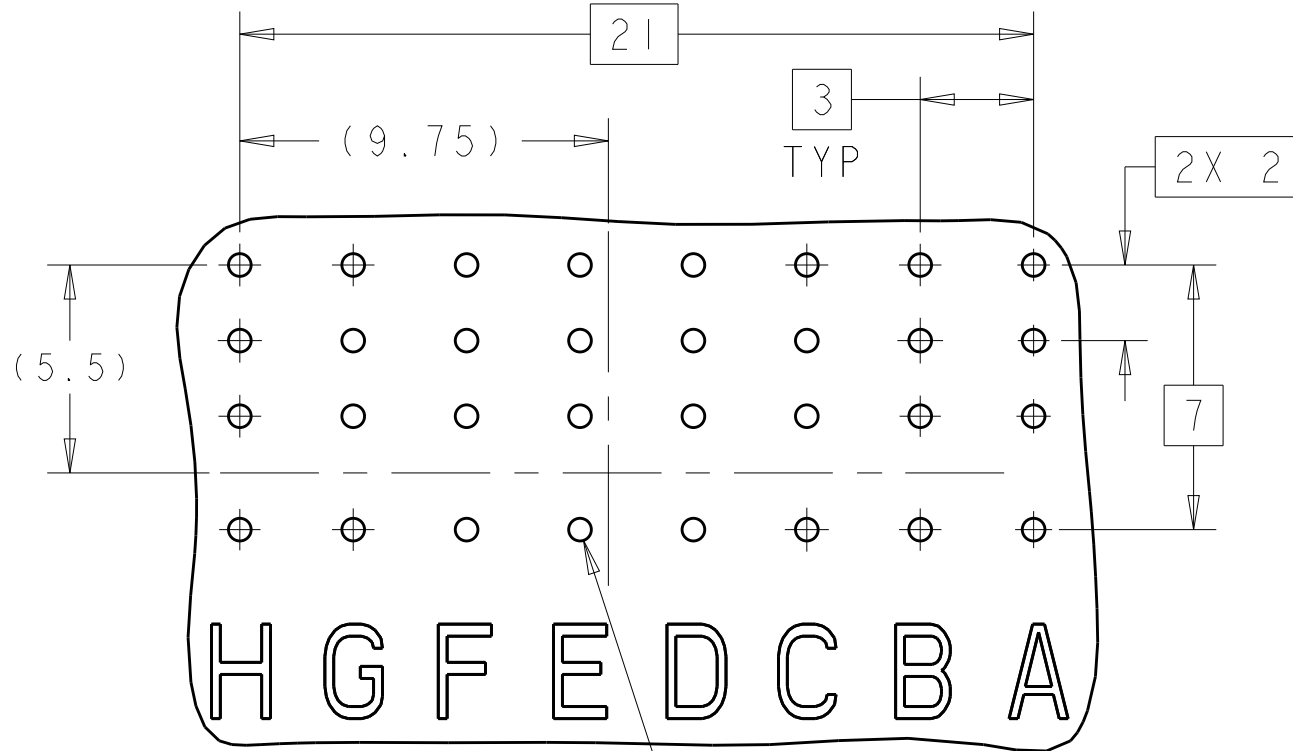
DETAIL K SCALE 5:1 8 POSITION UNIVERSAL POWER MODULE
