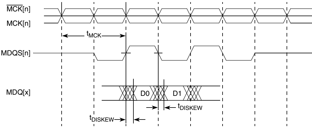
Figure 3. DDR SDRAM Input Timing Diagram ( t_{DISKEW} )
