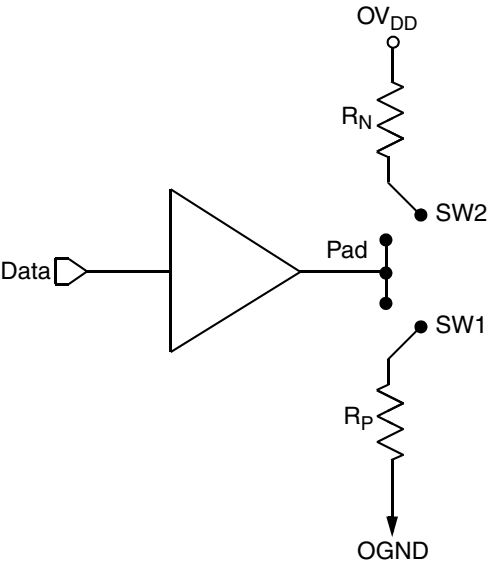
Figure 63. Driver Impedance Measurement
