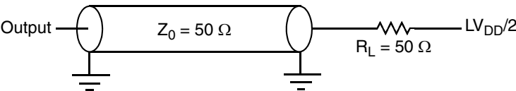
Figure 10. eTSEC AC Test Load
