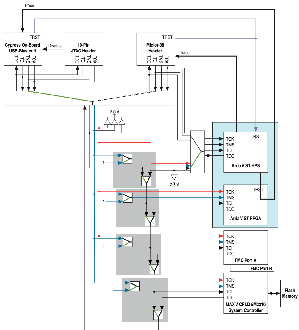
Figure 2-3. JTAG Chain
