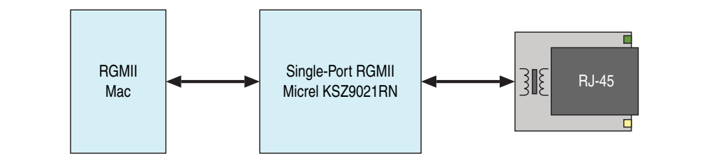
Figure 2-7. RGMII Interface between HPS (MAC) and PHY
