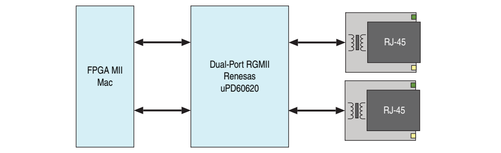
Figure 2–8. MII Interface between FPGA (MAC) and PHY
