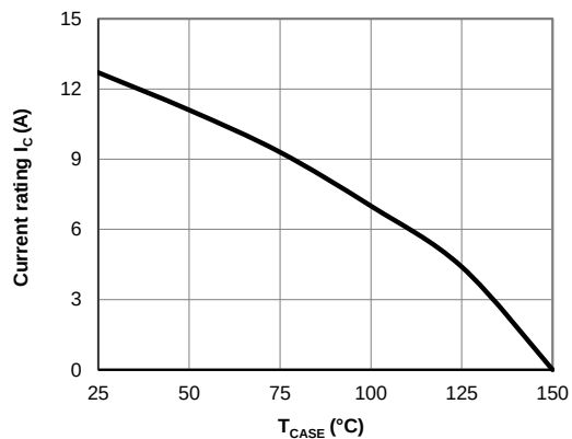
Figure 11: Current De-rating
