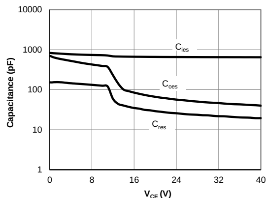
Figure 8: Capacitance Characteristic
