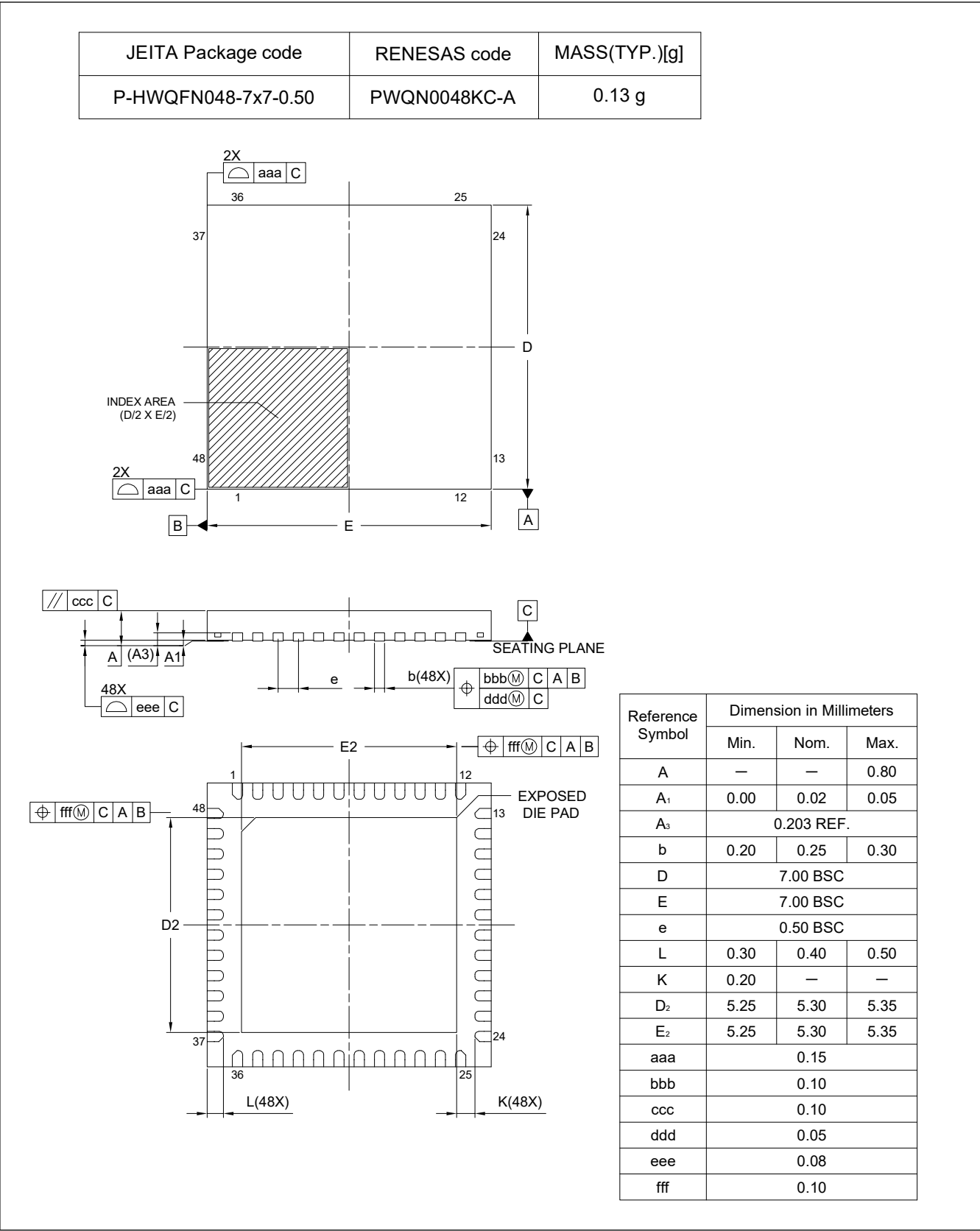
Figure A2.3 QFN 48-pin
