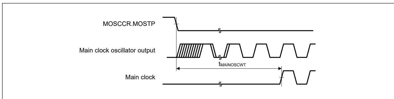
Figure 2.8 Main clock oscillation start timing
