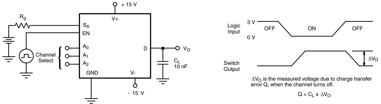
Fig. 5 - Charge Injection
