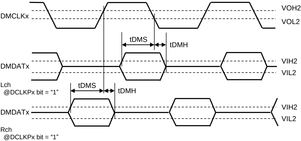
Figure 13. Audio Interface Timing
