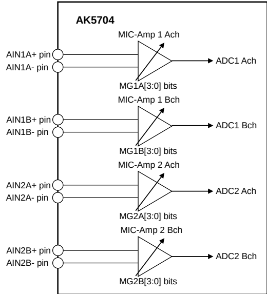
Figure 32. MIC Input Volume Setting
