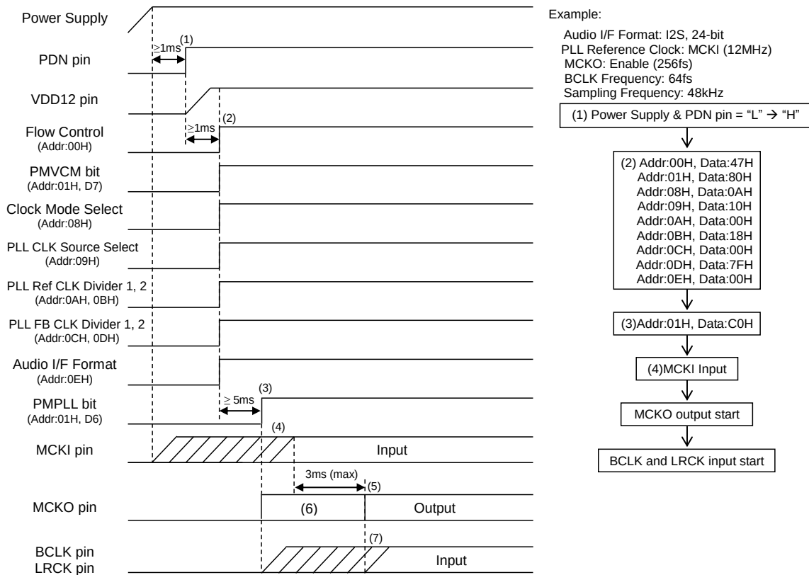
Figure 60. Clock Set Up Sequence (3)
