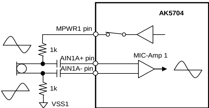
Figure 30. Connection Example for Full-differential Microphone Input
