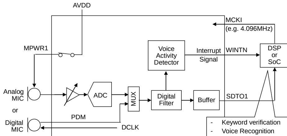
Figure 44. Voice Activity Detector System Block Diagram
