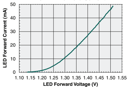
Typical LED Forward Voltage vs. LED Forward Current
