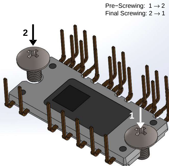
Figure 9. Mounting Screws Torque Order
