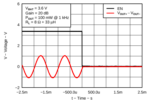
Figure 18. Shutdown timing
