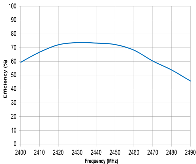
Efficiency
