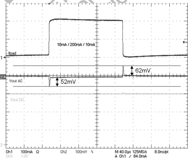
Figure 15. LDO3 Load Transient Response
