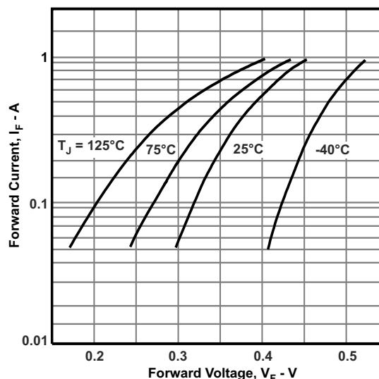
Figure 8-3. Diode Forward Characteristics MBR0530
